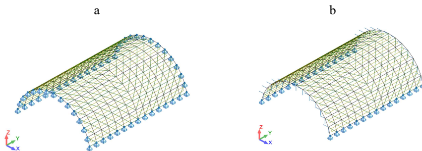
Fig. 11. The support conditions of the braced barrel vault with the Pratt type 1 bracing: a – the structure with all displacements fixed in the supports, b – the structure with displacement in y direction not fixed in the gable wall supports
